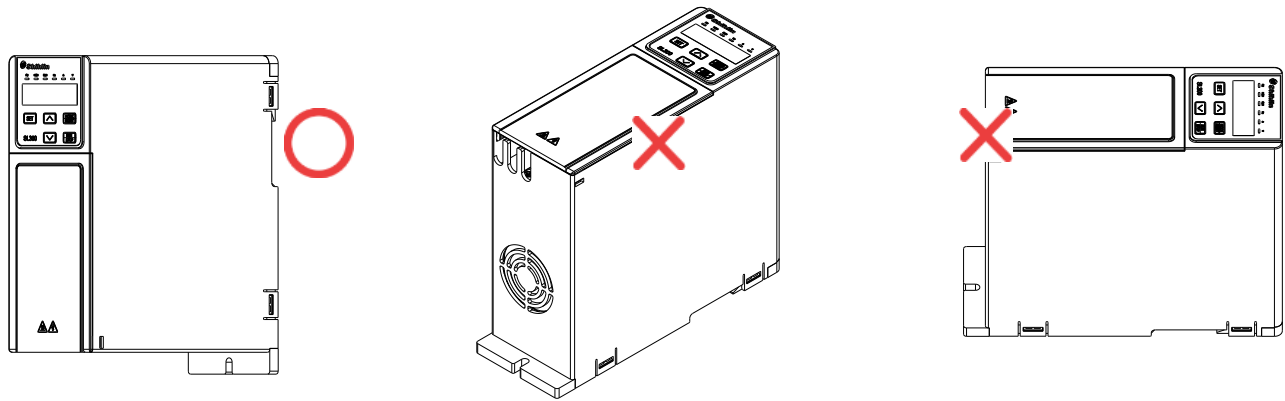
(a)纵向安装 (b)水平安装 (c)横向安装
